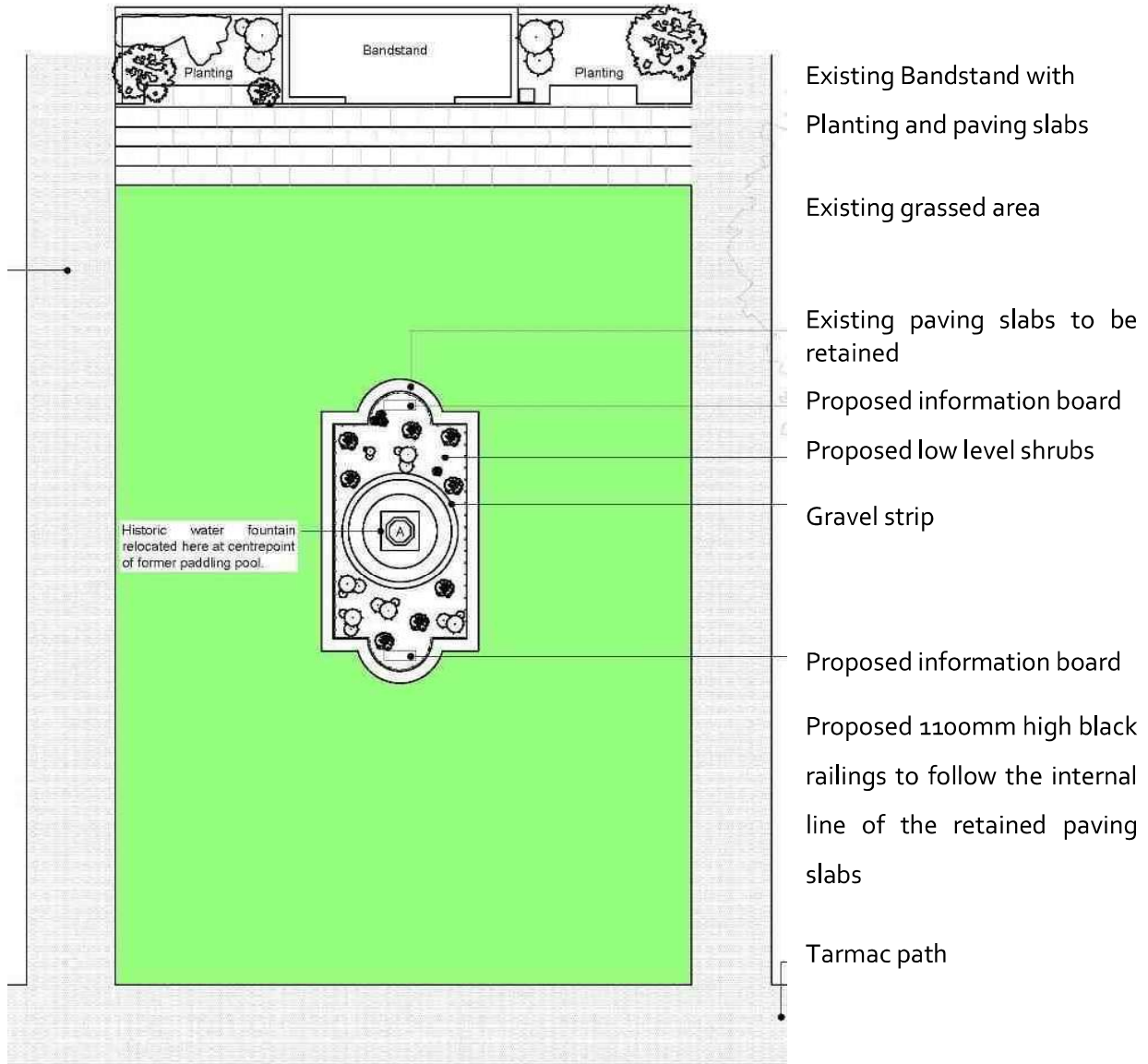
Image 23- Extract from Drawing A1572-02 Rev P2 – (Provided in the Appendices) showing the proposed position 3 of the fountain at the centre of the former paddling pool
